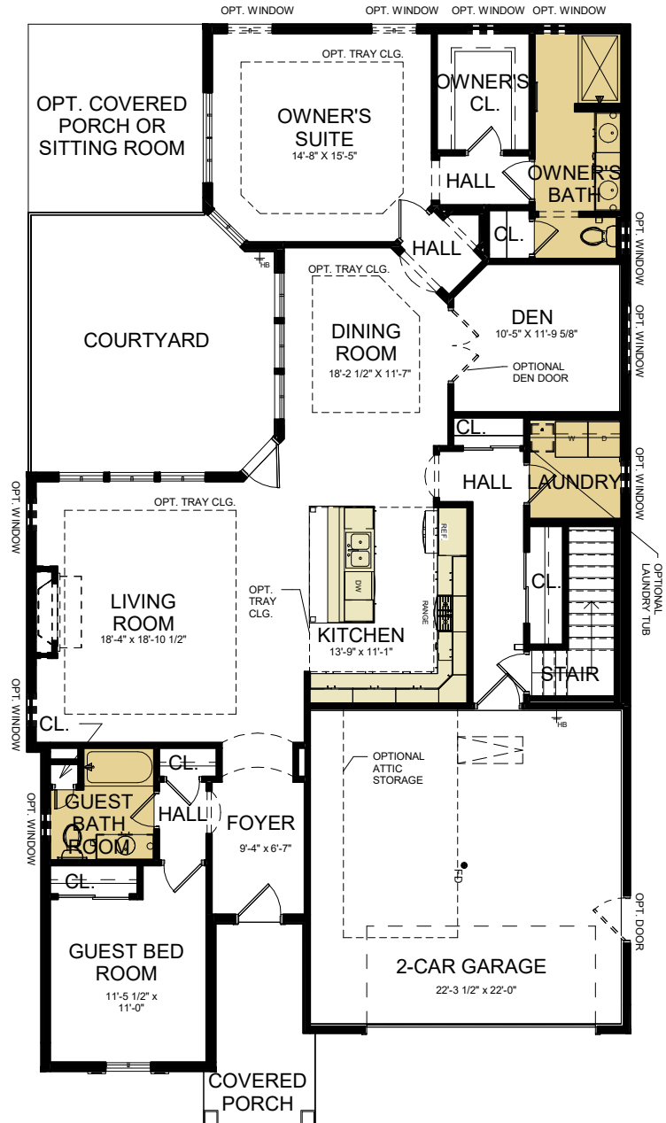
FIRST FLOOR PLAN WITH OPTIONAL BONUS SUITE
