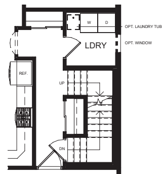
STAIR W/ BASEMENT & BONUS SUITE
