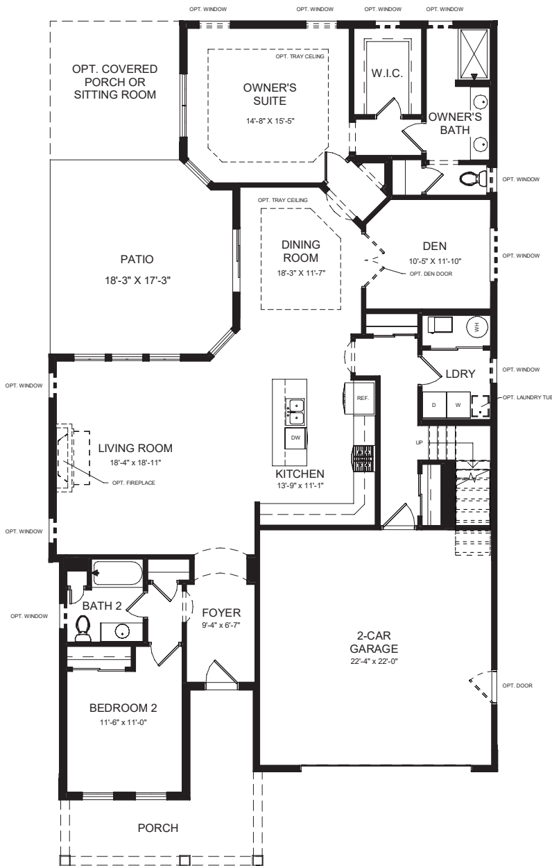
SINGLE LEVEL FLOOR PLAN W/ BONUS SUITE
