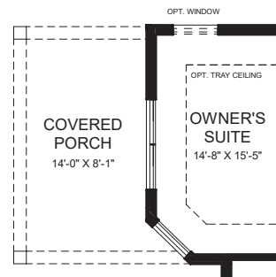
COVERED PORCH w/ WINDOWS I.L.O. SLIDER
