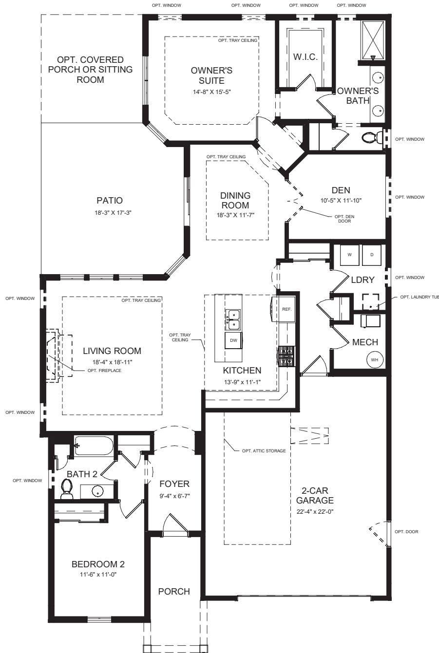
SINGLE LEVEL FLOOR PLAN
