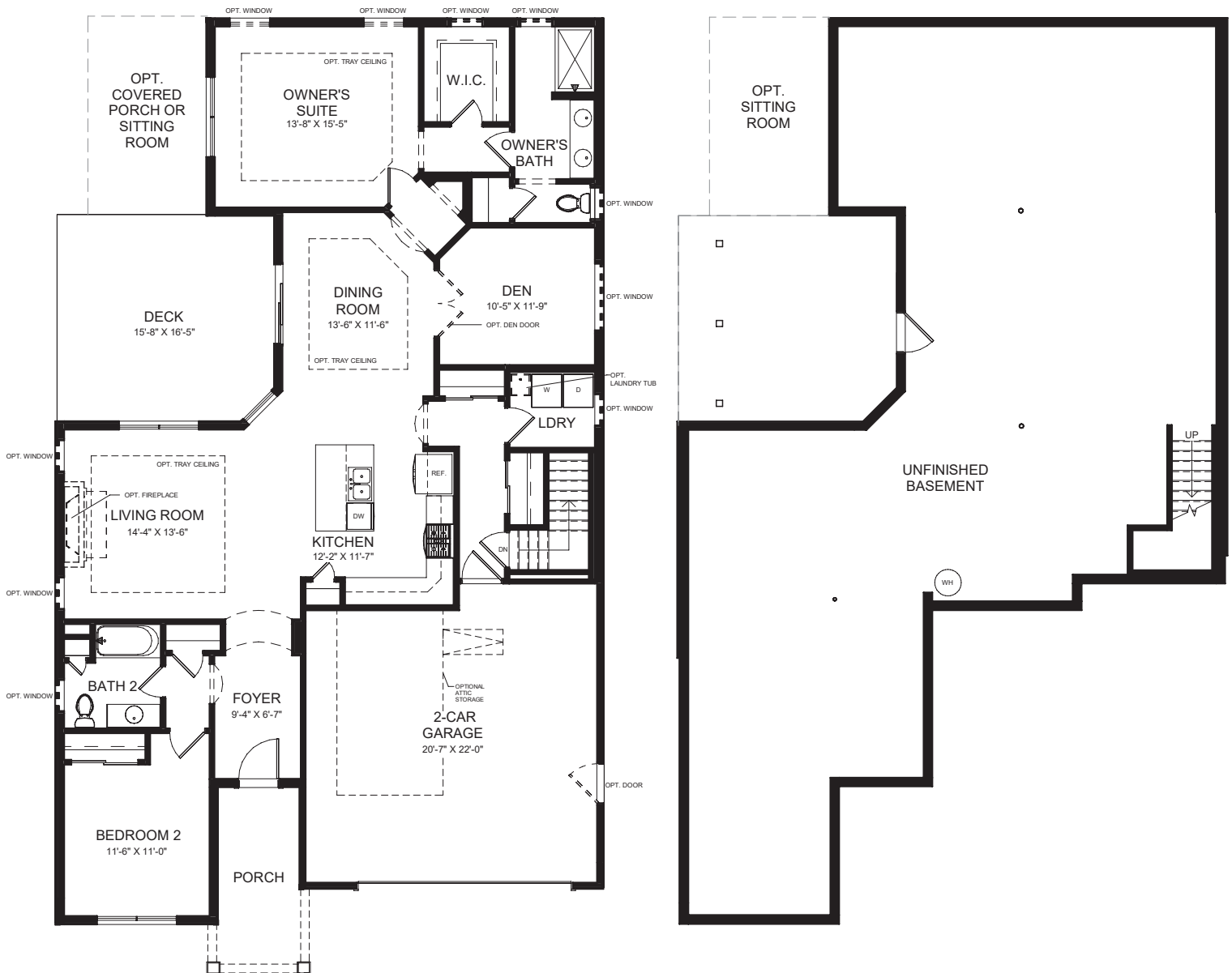
FIRST FLOOR PLAN W/BASEMENT
