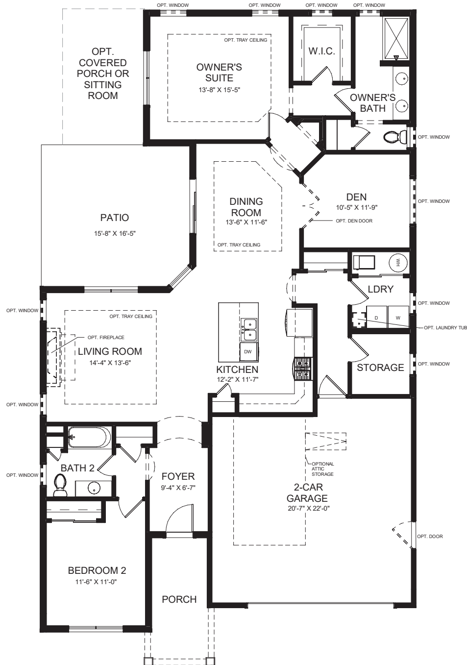
SINGLE LEVEL FLOOR PLAN
