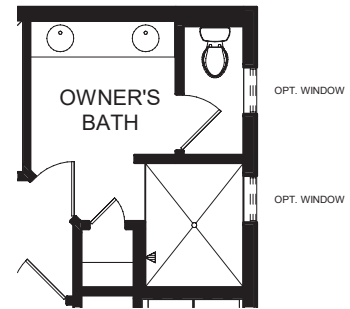
OWNER'S ZERO THRESHOLD SHOWER
