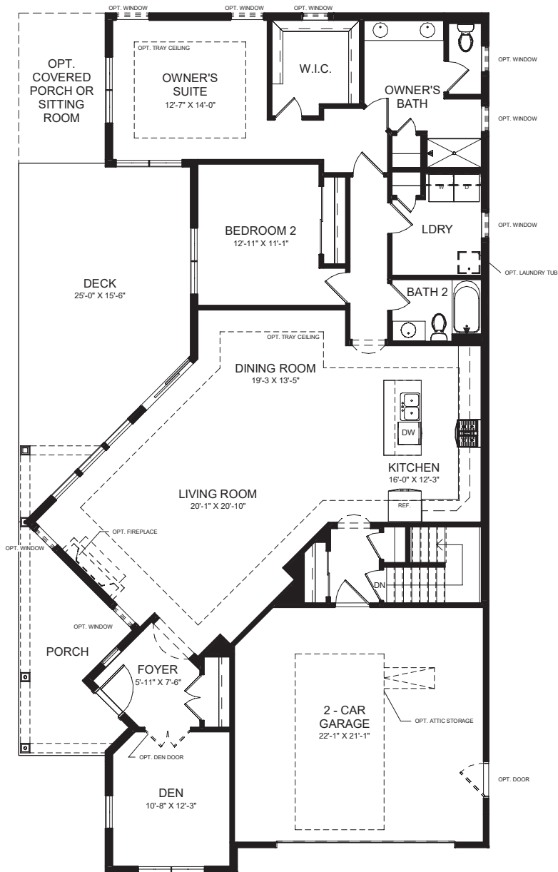
FIRST FLOOR PLAN W/BASEMENT
