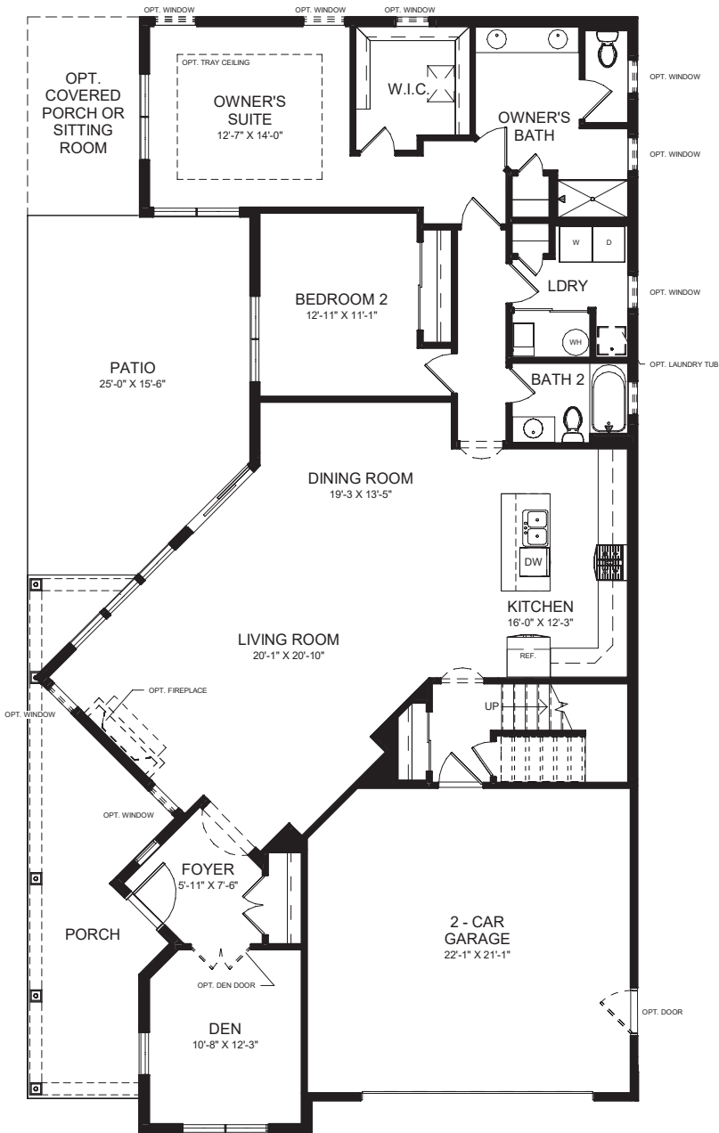
SINGLE LEVEL FLOOR PLAN W/ BONUS SUITE
