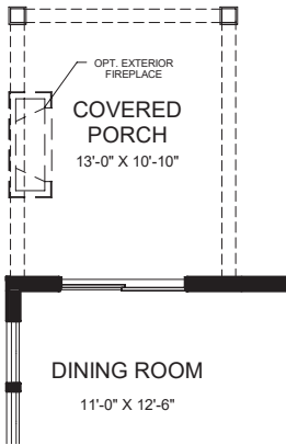
DINING ROOM COVERED PORCH
