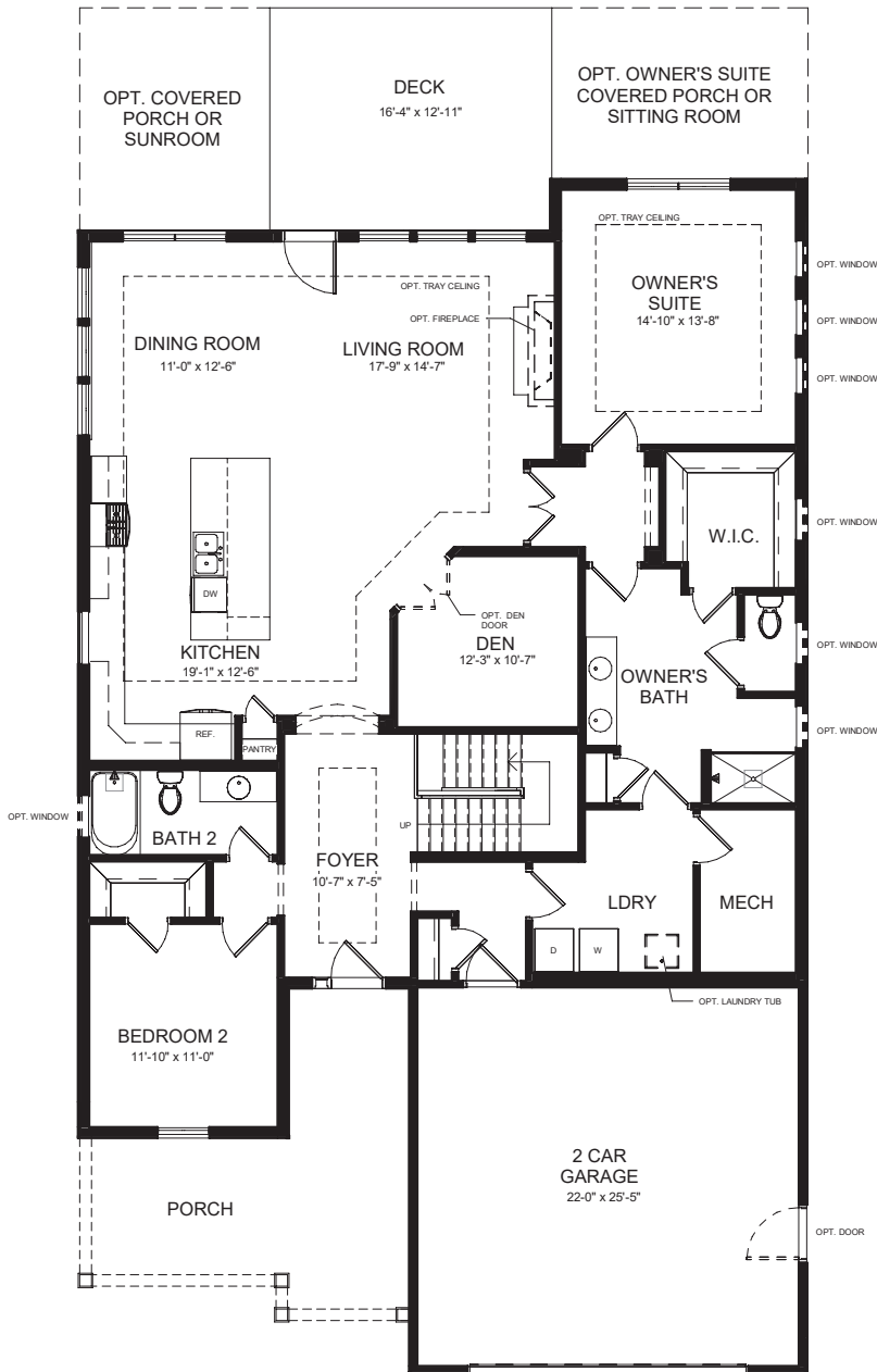
FIRST FLOOR PLAN W/FINISHED BASEMENT
