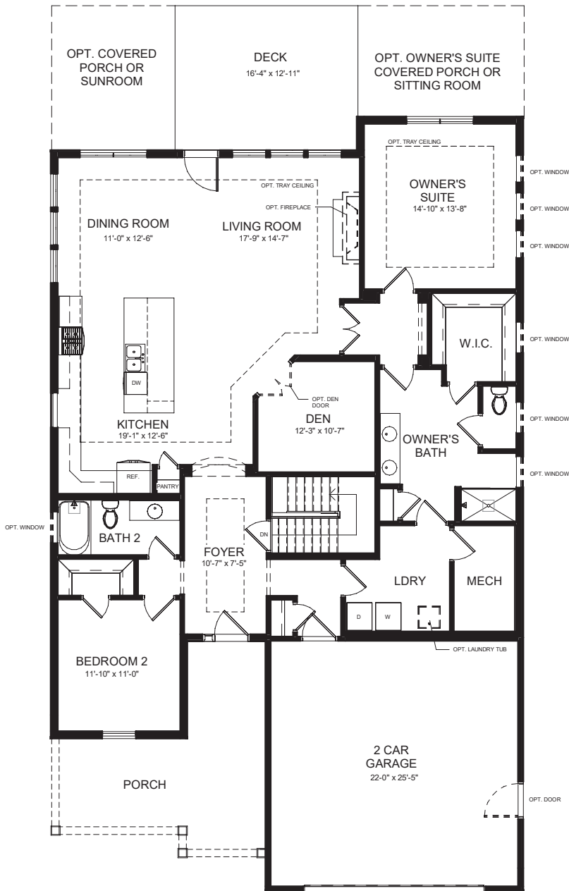
FIRST FLOOR PLAN W/UNFINISHED BASEMENT
