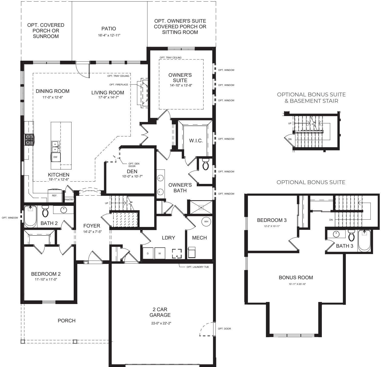
SINGLE LEVEL FLOOR PLAN W/ BONUS SUITE
