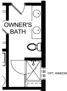
OWNER'S BATH DELUXE SHOWER
