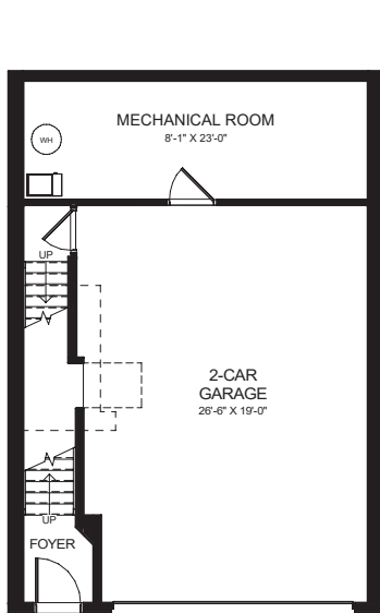
UNFINISHED BASEMENT
