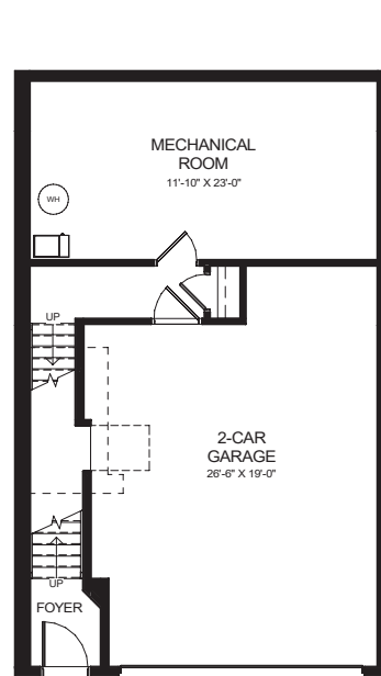
UNFINISHED BASEMENT
