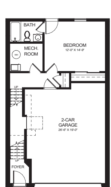
FINISHED BASEMENT W/ OPT. BEDROOM
