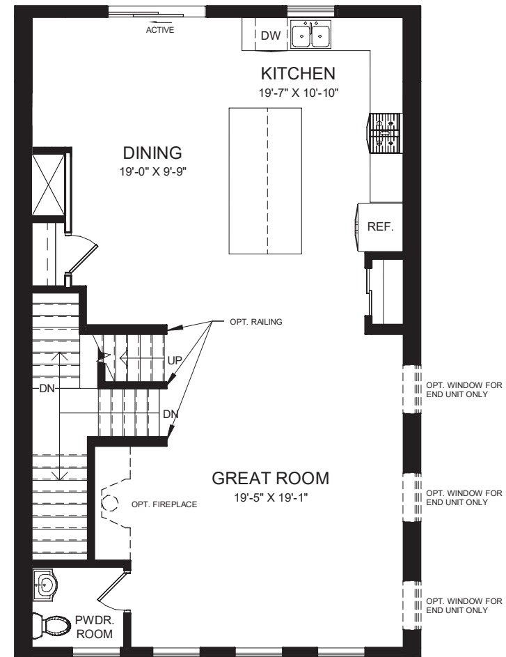
FIRST FLOOR REAR KITCHEN W/ 4' EXTENSION
