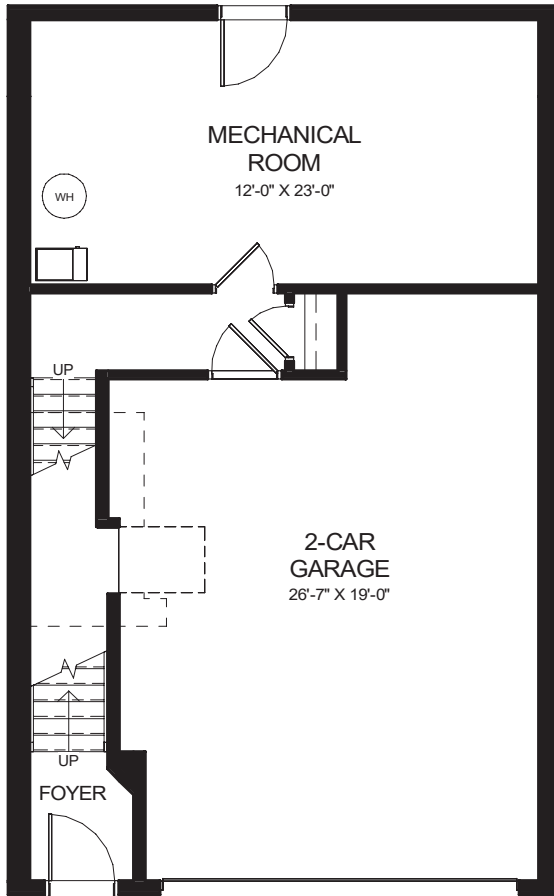
UNFINISHED BASEMENT
